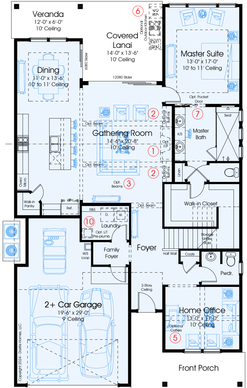
First Floor Plan - Coastal
