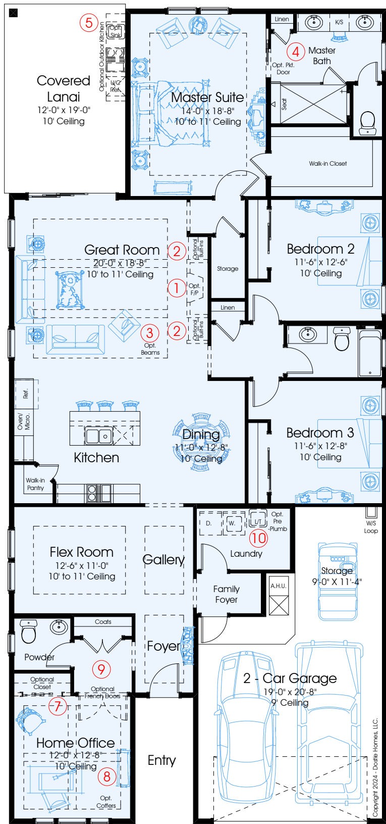
Floor Plan -Seaside
