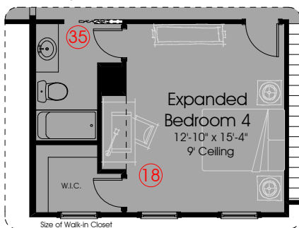
Optional Bathroom 6 and Expanded Bedroom 4 i.l.o. 2-Story Foyer and Entry
