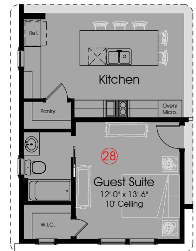
Optional Guest Suite w/ Full Bath i.o. Flex Room
