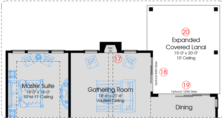
Optional Expanded Covered Lanai Optional Fireplace at Gathering Room
