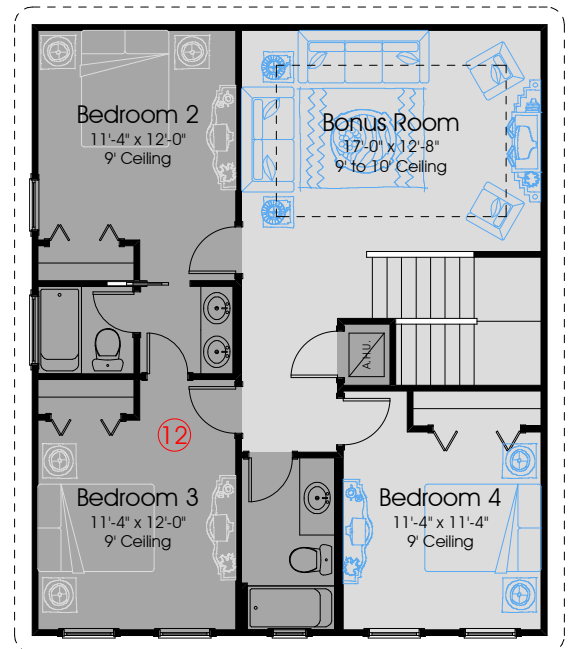
Optional Second Floor Plan
