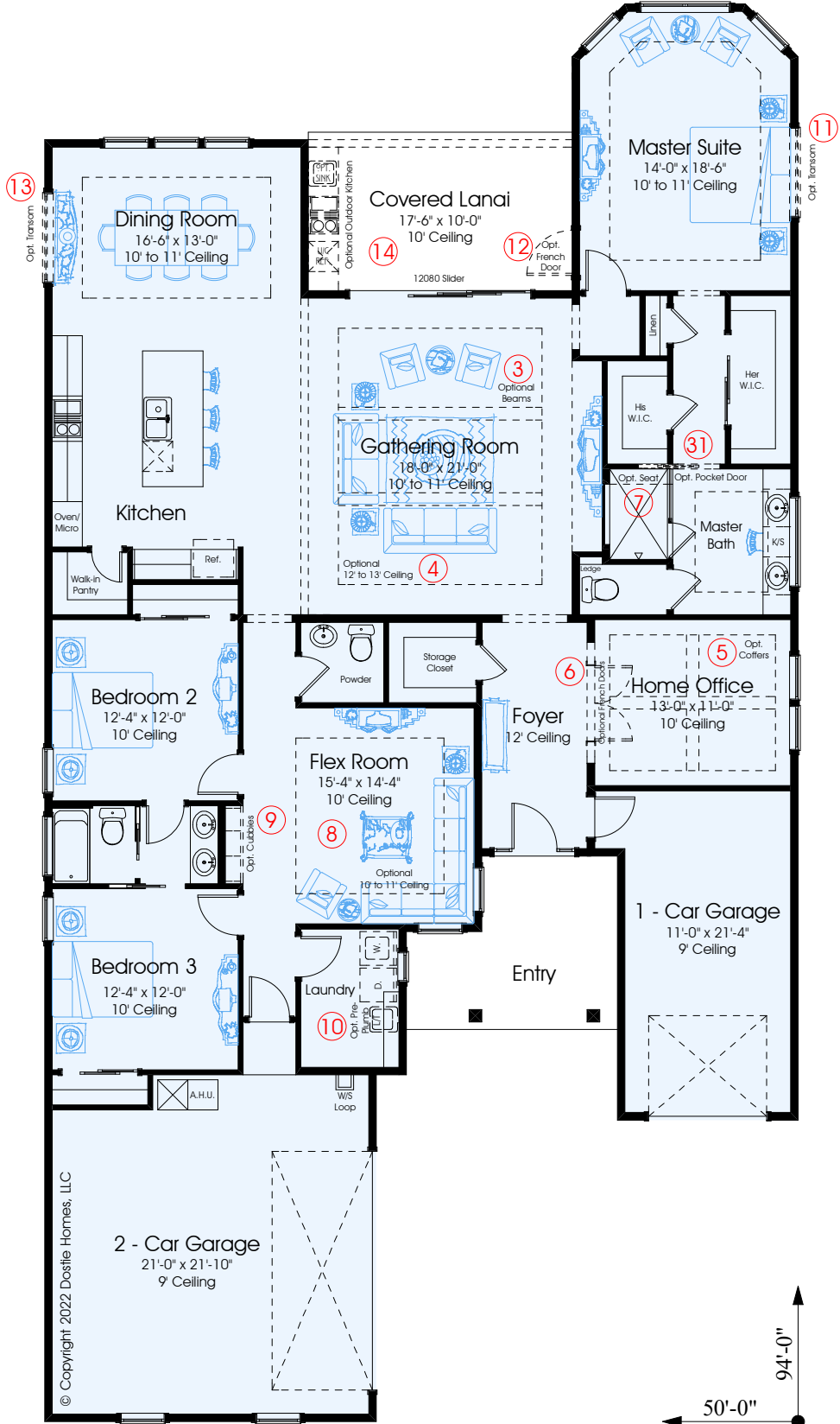
First Floor Plan - Seaside
