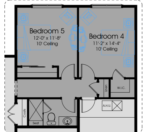
Optional Bedroom 5 i.l.o. Living Room (shown with shower i.l.o. tub)
